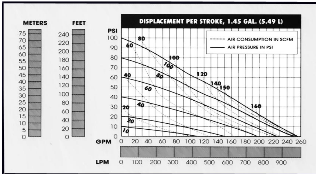
3" PERFORMANCE CURVE
